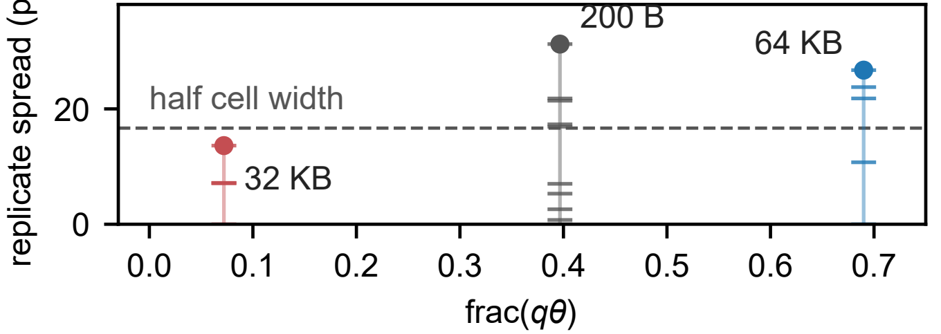
Fig. S5. Campaign’s confirmed prediction. (a) Retention replicates at 300 msg/s ( q = 3 ) by payload, against the thirds grid: 200 B straddles both branches, 32 KB pins near the 2/3 vertex, 64 KB re-opens to the upper cell. Horizontal position within an configuration separates replicates that would overprint and carries no variable. (b) Replicate spread against \text{frac}(q\theta) : the flat–full boundary at half the cell width is crossed in both directions by the one manipulated variable. The spread is a range, so each stick shows the replicates it is made of — 32 KB clears the boundary with three of five pinned together, 64 KB is broad.
