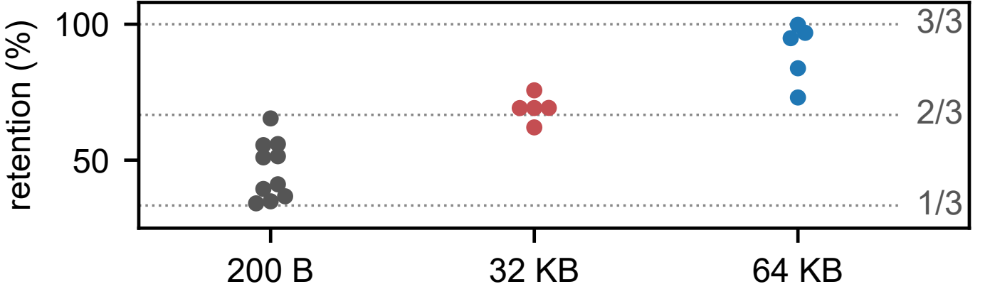
(a) Replicates against the q = 3 grid
