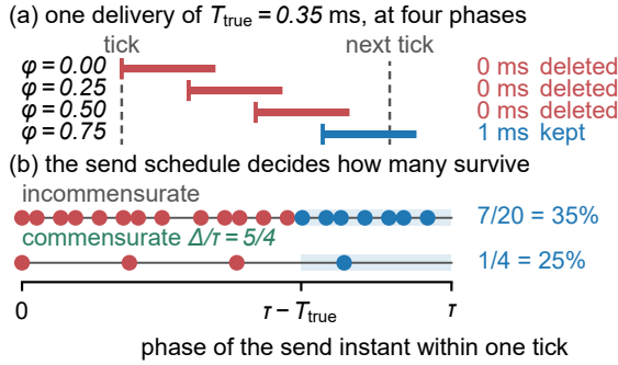
Fig. 4. Why a sample disappears, and why the survivors are not a sample. (a) One delivery of T_{\text{true}} = 0.35 ms at four phases of one tick. Three finish inside it, so both stamps round alike, the difference is exactly zero, and the guard removes them; the fourth crosses the boundary and is recorded as one whole tick — which is why the corpus prints 1.0 and 2.0 ms and nothing between. (b) A delivery survives from phase \tau - T_{\text{true}} onward — the shaded band — so uniform phases retain T_{\text{true}}/\tau (Equation 4); a commensurate producer visits only q and retains a count out of q , one of the values Equation 5 allows. T_{\text{true}} here is illustrative and off-vertex by choice: at 0.5 ms the two answers coincide.
