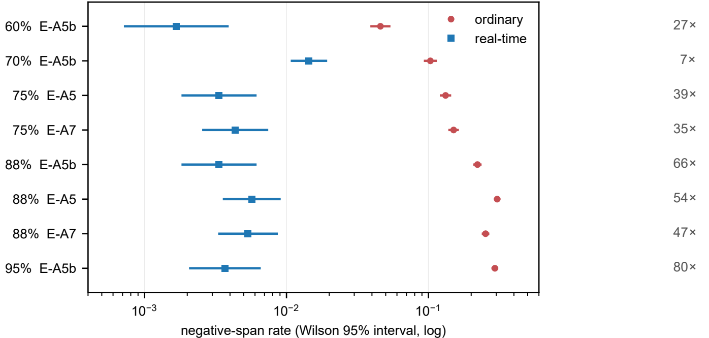
Fig. 9. The same 8 pairs, as a ladder. Ordinary and real-time negative-span rates with Wilson 95% intervals, one row per pair, ordered by achieved utilization; the factor is printed at the right. Reading down, the real-time arm barely moves while the ordinary arm climbs with load, which is what makes the factor grow. The growth is a trend and not a law — 60% gives 27\times and 70% gives 7\times — and the range is reported as a range for that reason.
