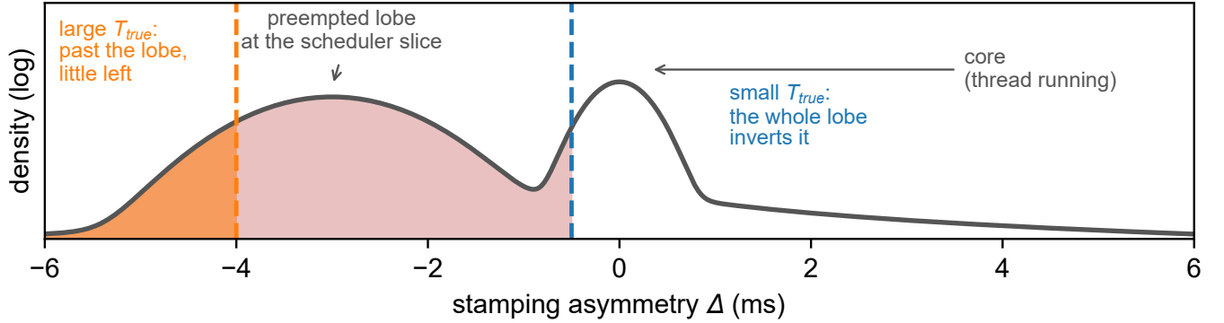
Fig. 3. The two-state model, drawn. The timestamping asymmetry \Delta has a narrow core when the timestamping thread is running and a lobe at -3 ms, the scheduler's base slice, when it is not, so a small T_{\text{true}} is inverted by the whole lobe and a large one only by what lies beyond it — which is why the check bites hardest on small effects. The shape is schematic, two components placed at the measured mode's location rather than a fit; the measured distribution is the traced stall spectrum of the main text.
