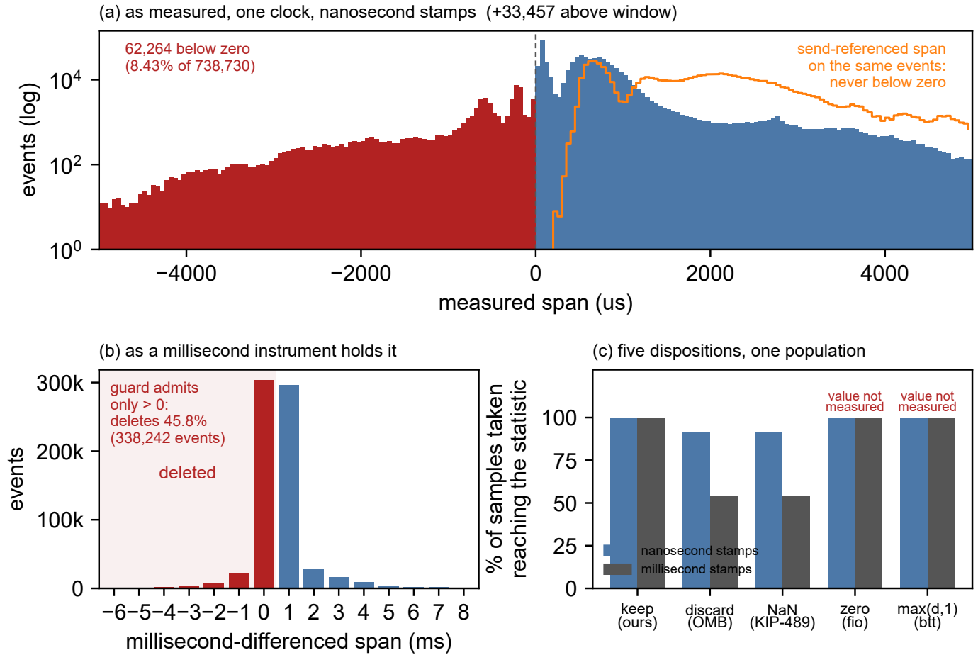
Fig. 8. What the instrument deletes, beside what it then reports. (a) At nanosecond resolution the acknowledgment-referenced span goes below zero 62,264 times in 738,730; the send-referenced span, same events and same clock, never does. (b) A millisecond instrument cannot see (a): it differences two truncated timestamps, so a sub-millisecond flight lands on 0 or 1 by tick alignment alone, and a positivity guard then deletes 45.8% of the population uncounted. (c) The five dispositions found in shipping software (Section S36), applied to that same population. Every count is emitted from the committed corpus by scripts/span_histogram.py .
