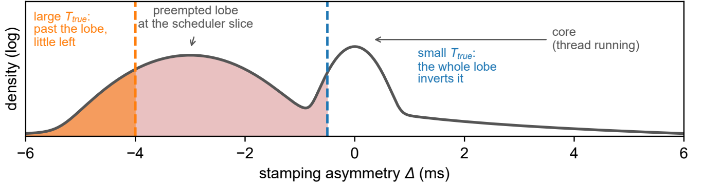
Fig. 4. The two-state model, drawn. The timestamping asymmetry \Delta has a narrow core when the timestamping thread is running and a lobe at -3 ms, the scheduler’s base slice, when it is not, so a small T_{\text{true}} is inverted by the whole lobe and a large one only by what lies beyond it — which is why the check bites hardest on small effects. The shape is schematic, two components placed at the measured mode’s location rather than a fit; the measured distribution is the traced stall spectrum of the main text.
