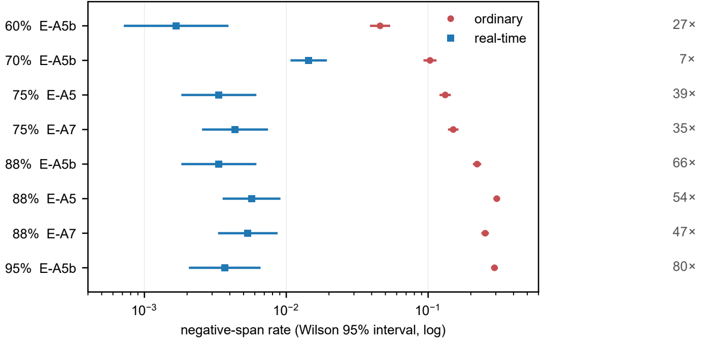
Fig. 6. The same 8 pairs, as a ladder. Ordinary and real-time negative-span rates with Wilson 95% intervals, one row per pair, ordered by achieved utilization; the factor is printed at the right. Reading down, the real-time configuration barely moves while the ordinary configuration climbs with load, which is what makes the factor grow. The growth is a trend and not a law — 60% gives 27 \times and 70% gives 7 \times — and the range is reported as a range for that reason.
