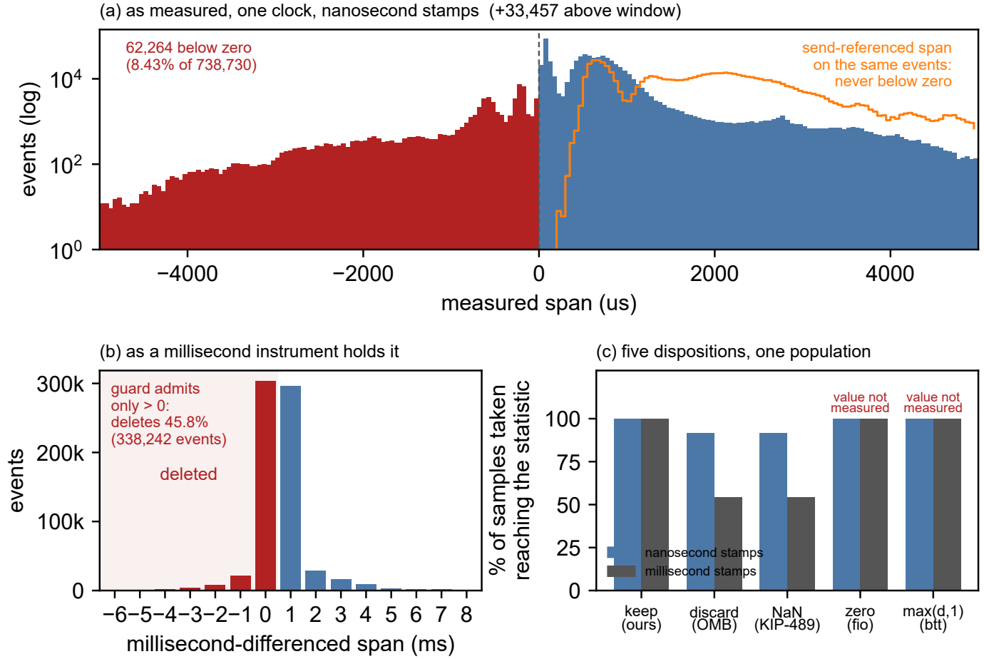
Fig. 10. What the benchmark deletes, beside what it then reports. (a) At nanosecond resolution the acknowledgment-referenced span goes below zero 62,264 times in 738,730; the send-referenced span, same events and same clock, never does. (b) A millisecond timestamp cannot see (a): it differences two truncated timestamps, so a sub-millisecond delivery lands on 0 or 1 by tick alignment alone, and an admission condition then deletes 45.8% of the population uncounted. (c) The five dispositions found in shipping software (Section S37), applied to that same population. Every count is emitted from the committed corpus by scripts/span_histogram.py .
