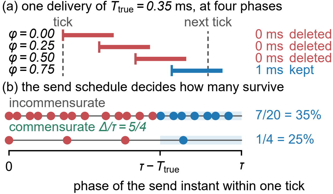
Fig. 11. Why a sample disappears, and why the survivors are not a sample. (a) One delivery of T_{\text{true}} = 0.35 ms at four phases of one tick. Three finish inside it, so both timestamps round alike, the difference is exactly zero, and the admission condition removes them; the fourth crosses the boundary and is recorded as one whole tick — which is why the corpus prints 1.0 and 2.0 ms and nothing between. (b) A delivery survives from phase \tau - T_{\text{true}} onward — the shaded band — so uniform phases retain T_{\text{true}}/\tau (Equation 4); a commensurate producer visits only q and retains a count out of q , one of the values Equation 5 allows. T_{\text{true}} here is illustrative and off-vertex by choice: at 0.5 ms the two answers coincide.
