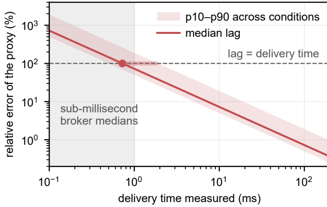
Fig. 5. Where a path sits on the exposure curve. The proxy's error A/D against the delivery time measured, the line at the median lag. Across conditions A runs 500–1900 \mu\text{s} between its tenth and ninetieth percentiles, the band, which puts the error at 10 ms at 5–19% and the crossover at 0.50–1.90 ms. On the dashed line, which the median crosses at 0.72 ms, the lag is as long as the path itself, and the shaded decade holds the sub-millisecond medians brokers now publish. A harness that times from the send subtracts no lag and has no curve.
