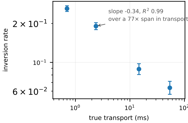
Fig. 7. A longer interval inverts less often. Inversion rate against true transport over the payload sweep, Wilson 95% intervals. The same stall distribution overlaps a short interval almost entirely and a long one hardly at all, which is Equation 3 as an experiment: lengthening what is being measured lowers the rate, where a load-driven account predicts no change.
