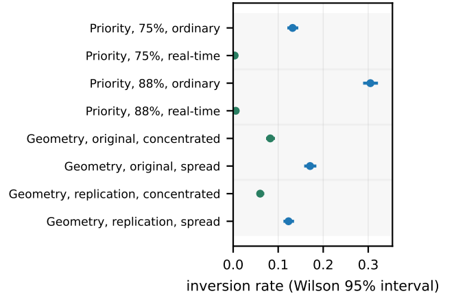
Fig. 6. Every manipulation, and no overlap. Wilson 95% intervals for the four matched pairs of Table IV: real-time priority against ordinary at two utilisations, and concentrated against spread geometry at equal \rho in two campaigns. Utilisation is held fixed within each pair, so what moves the rate is where the stamping thread sits, not how loaded the machine is.
