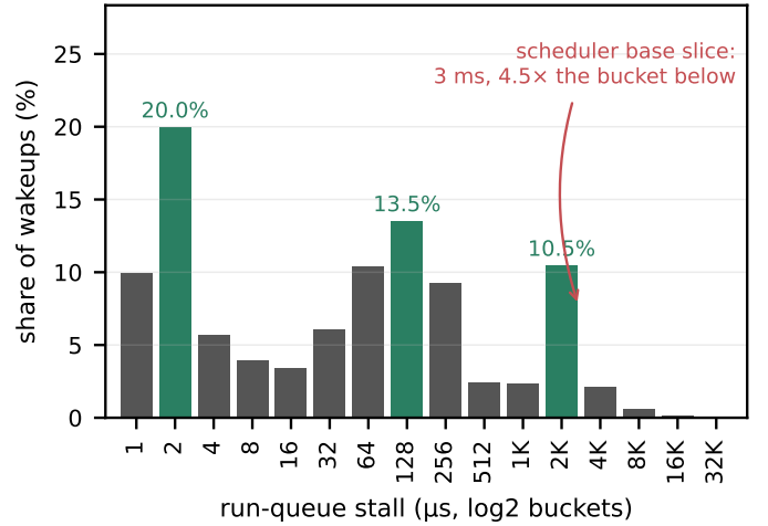
Fig. 8. The traced run-queue stall distribution is trimodal. 551,956 wakeups, bpfttrace log 2 buckets, modes shaded. The jitter core sits at a few microseconds and a second mode at 128–256 μs; the third, holding 10.5% of all wakeups, lands on the scheduler’s derived base slice of 3 ms. A power law would have to descend monotonically across this axis.
