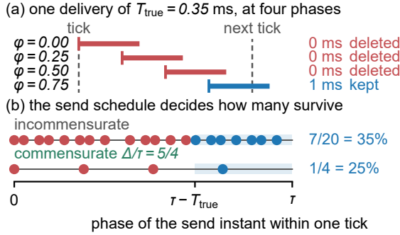
Fig. 3. Why a sample disappears, and why the survivors are not a sample. (a) One delivery of T_{\text{true}} = 0.35 ms at four phases of one tick. Three finish inside it, so both stamps round alike, the difference is exactly zero, and the guard removes them; the fourth crosses the boundary and is recorded as one whole tick — which is why the corpus prints 1.0 and 2.0 ms and nothing between. (b) A delivery survives from phase \tau - T_{\text{true}} onward — the shaded band — so uniform phases retain T_{\text{true}}/\tau (Equation 4); a commensurate producer visits only q and retains a count out of q , one of the values Equation 5 allows. T_{\text{true}} here is illustrative and off-vertex by choice: at 0.5 ms the two answers coincide.
