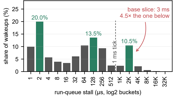
Fig. 3. Traced run-queue stalls are trimodal. 551,956 wakeups, bpfttrace log 2 buckets, modes shaded. The jitter core peaks in the 2–4 \mu\text{s} bucket, which alone holds 20.0% of all wakeups; a second mode at 128–256 \mu\text{s} holds 13.5%; the third, at 10.5%, lands on the scheduler’s derived base slice of 3 ms. A power law of any index above one would have to descend monotonically across this axis. The count survives a 2 \times widening of the buckets in both phasings, so it is not an artifact of where this tool put its edges.
