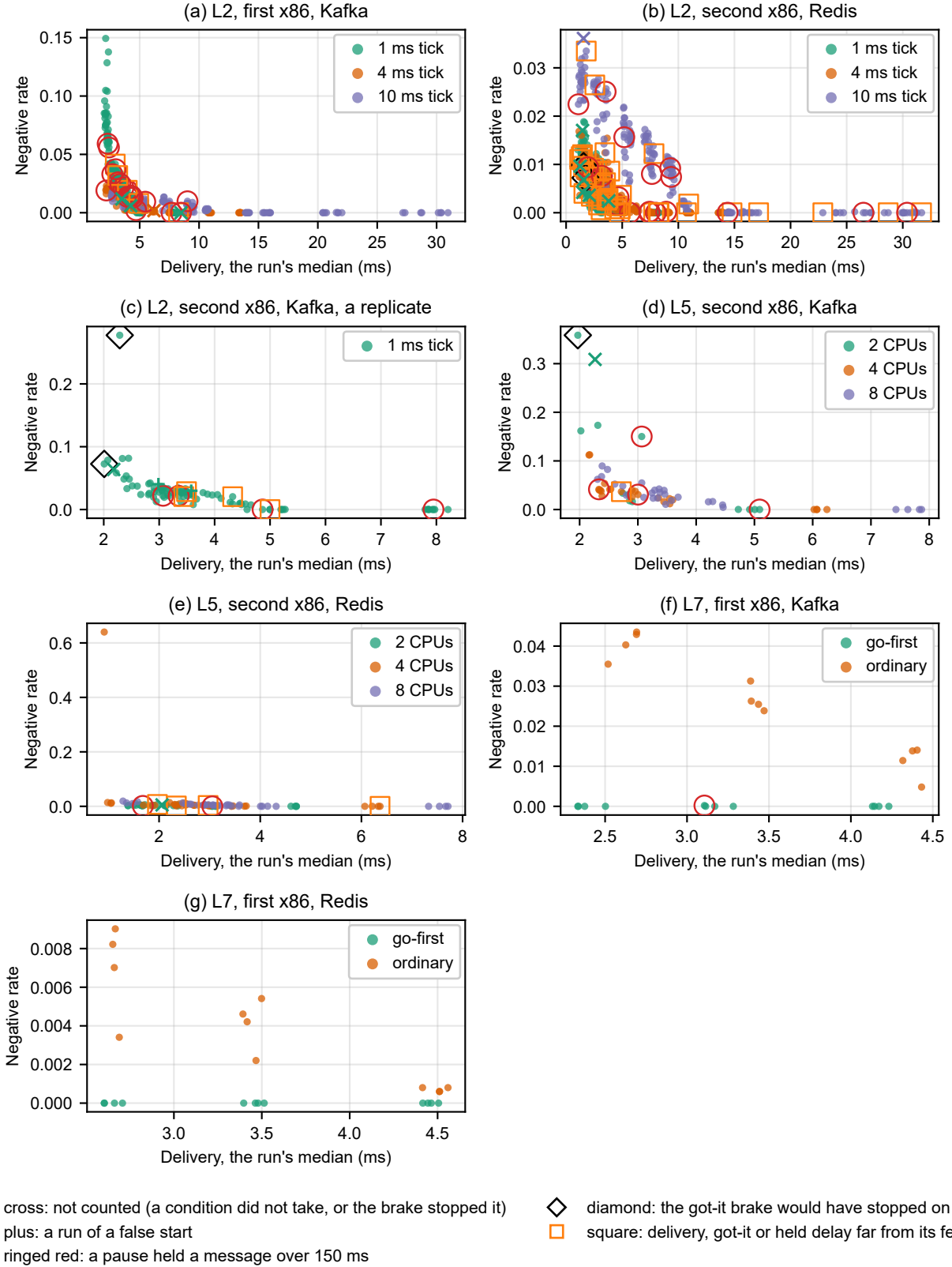
Fig. S17. Every tick, core-count and priority run, aberrant runs marked. L2 on the first x86 pair (Kafka) and the second (Redis), colored by the tick, the bridge days on the stock kernel with the 1 ms builds; in (c), the Kafka sessions the second pair ran on the 1 ms build before L2's Kafka half moved to the first pair, a replicate that no judgment pools with the first pair's runs; L5 on the second x86 pair, colored by the online CPUs; L7 on the first, ordinary against real-time priority. Marks as in Figure S16.
