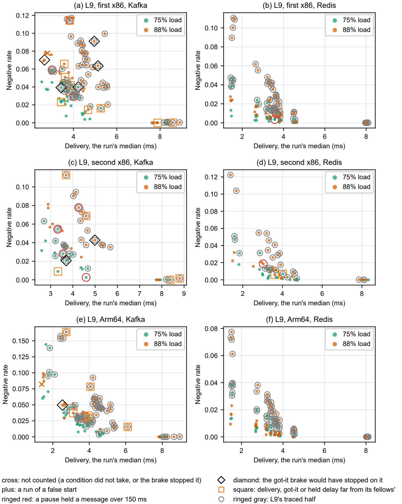
Fig. S19. Every L9 run, aberrant runs marked. Both brokers on all three pairs, colored by load; gray rings mark the traced half, whose event tracer raised the rate it recorded. Other marks as in Figure S16.
