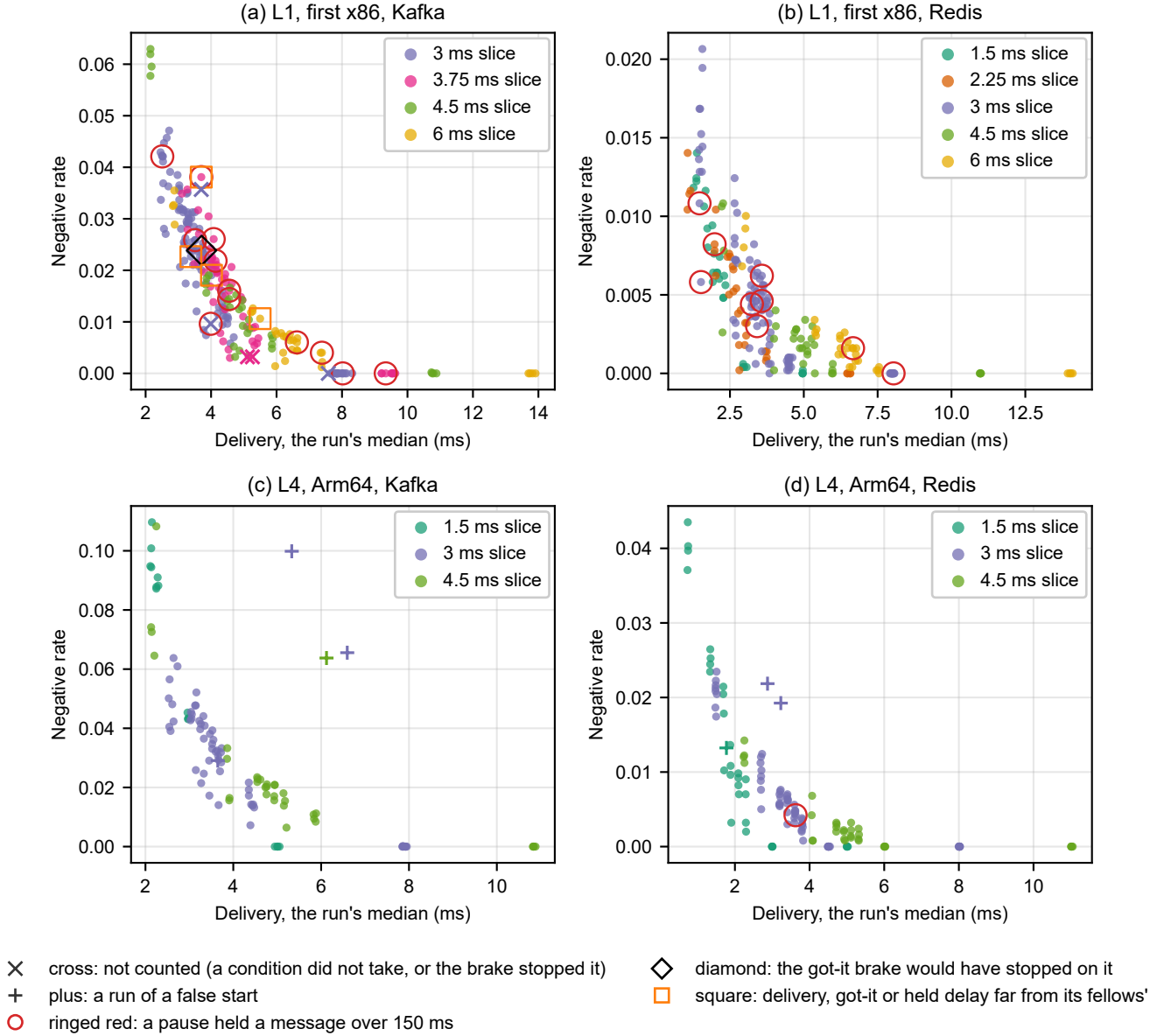
Fig. S16. Every slice run, aberrant runs marked. Each run of L1 (first x86 pair) and L4 (Arm pair, Arm64 in the panels) at its median delivery and its negative-span rate, colored by the slice it ran at. Crosses: runs the integrity rule did not count. Plusses: runs of L4's two false starts. Rings: counted runs with a warning, each reason its own shape (Table S31).
