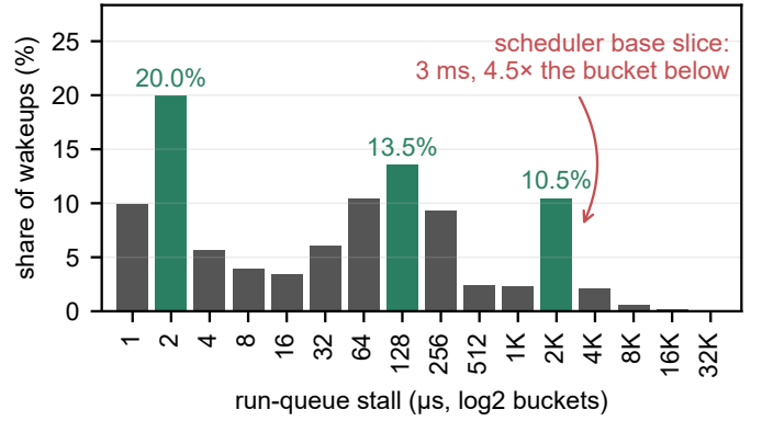
Fig. 7. The traced run-queue stall distribution is trimodal. 551,956 wakeups, bpfttrace \log_2 buckets, modes shaded. The jitter core sits at a few microseconds and a second mode at 128\text{--}256\mu\text{s} ; the third, holding 10.5% of all wakeups, lands on the scheduler's derived base slice of 3 ms. A power law would have to descend monotonically across this axis.
