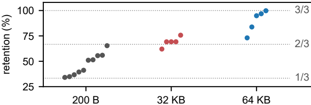
(a) replicates against the q = 3 grid
