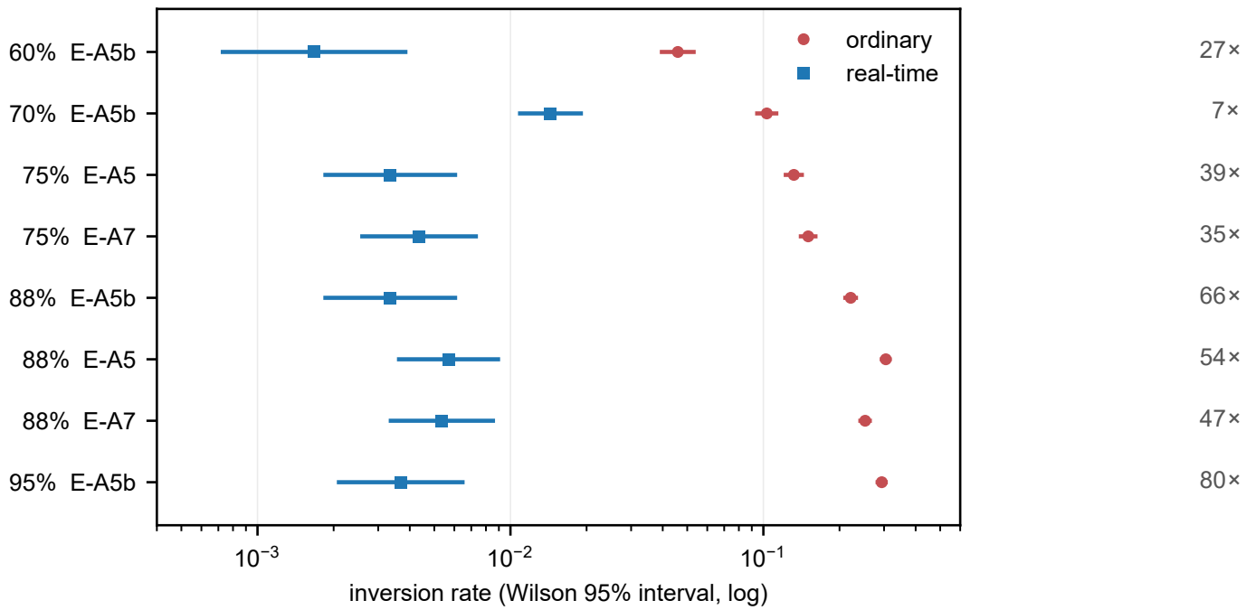
Fig. 6. The same 8 pairs, as a ladder. Ordinary and real-time inversion rates with Wilson 95% intervals, one row per pair, ordered by achieved utilization; the factor is printed at the right. Reading down, the real-time arm barely moves while the ordinary arm climbs with load, which is what makes the factor grow. The growth is a trend and not a law — 60% gives 27× and 70% gives 7× — and the range is reported as a range for that reason.
