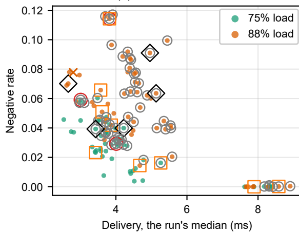
(c) A9, second x86, Kafka
