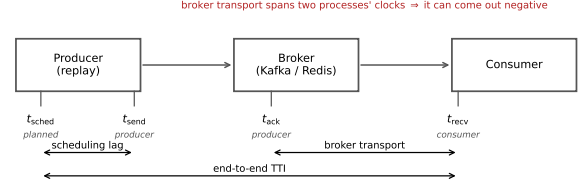
Figure 1: The four timestamps and the intervals each measure spans. Scheduling lag is measured within one process. Broker transport subtracts a producer-side timestamp from a consumer-side one, and can therefore come out negative when either process is delayed.
