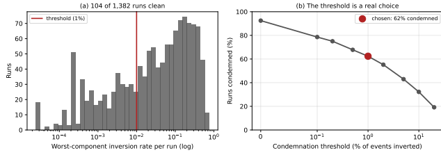
Figure 2: The audit on Testbed A. (a) Per-run inversion rates: 104 runs are clean and the rest spread over three decades, so there is no natural threshold. (b) Share of runs rejected against the threshold. The choice matters for the run count and not for any conclusion.
