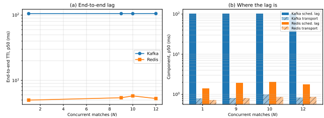
Figure 3: (a) End-to-end delay against concurrency, Testbed B, after the check. (b) The same runs decomposed: the twenty-fold difference is entirely producer scheduling lag, while the brokers’ own transport is separated by well under a millisecond. Log scale.
