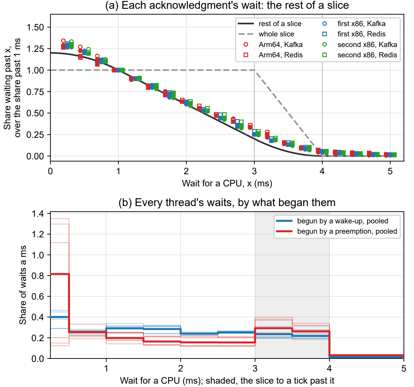
Fig. S12. Each acknowledgment waits out the rest of a slice, not a whole one. (a) For every acknowledgment in A9's recorded runs on the three pairs, the share whose timestamping thread was still waiting for a CPU at each wait x , over the share still waiting at 1 ms, for each pair, broker and load (open marks 75% load, filled 88%; Arm64 is the Arm pair; each pair's marks are set a little to one side of the wait they are read at); lines, the rest-of-a-slice shape of Equation S5 (solid) and the whole-slice shape of Equation S4 (dashed), at the 3 ms slice and 1 ms tick. (b) Every python3 thread's waits over 0.25 ms, as a share per millisecond in each bin, by what began them, each pair and broker thin and the six pooled bold; shaded, the slice to a tick past it.
