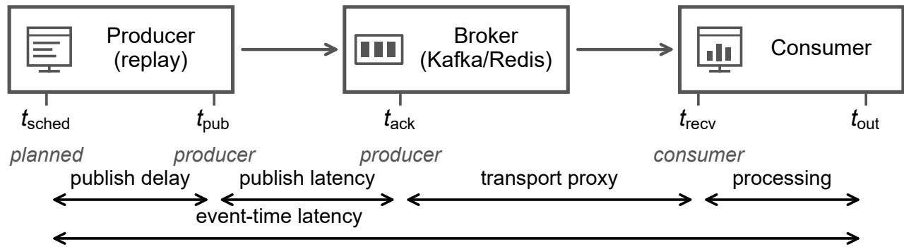
Fig. S16. System measured, and where its clocks are read. A replay process paces recorded match events at a chosen rate into a broker — Kafka or Redis Streams — and a consumer reads them back. The five timestamps and the five spans they bracket are those of main-text Section IV-A; the upper four are the terms of Equation 2 and sum to the fifth, the event-time latency, which the harness closes at t_{\text{out}} . The transport proxy subtracts a producer-process timestamp from a consumer-process one. Both processes run on one host reading one clock unless stated otherwise, so nothing drawn here depends on clock synchronization.
