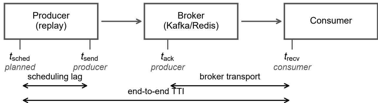
Fig. 9. The four timestamps, and the span each metric covers. Scheduling lag is measured inside one process. Broker transport subtracts a producer-side stamp from a consumer-side one, so it can come out negative when either process is delayed.
