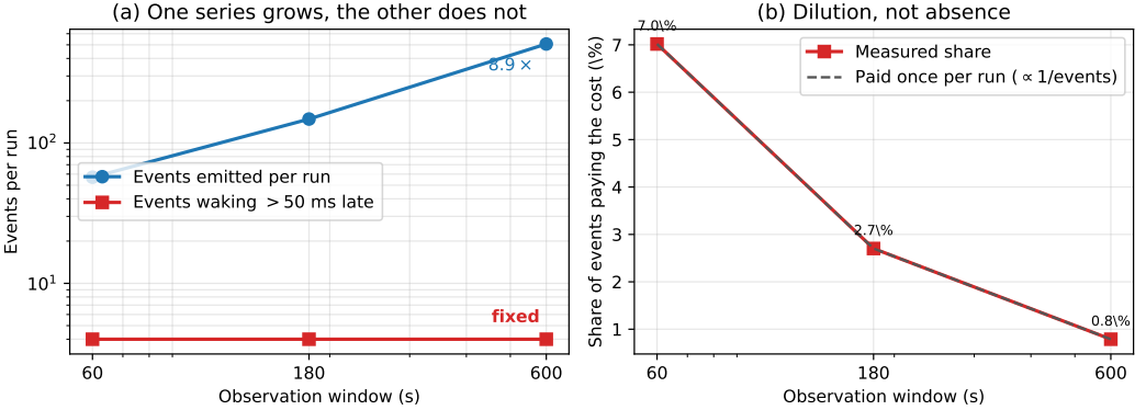
Fig. 4. The window sweep, as a picture. (a) Events emitted per run grow 8.9\times while the number waking more than 50 ms late stays at four — a per-event constant would put the two series on parallel lines. (b) The same fact as a proportion: the share of events paying the cost falls as 1/\text{events} , the dilution a once-per-run cost predicts. Redis, on the same events, has no affected events at any window.
