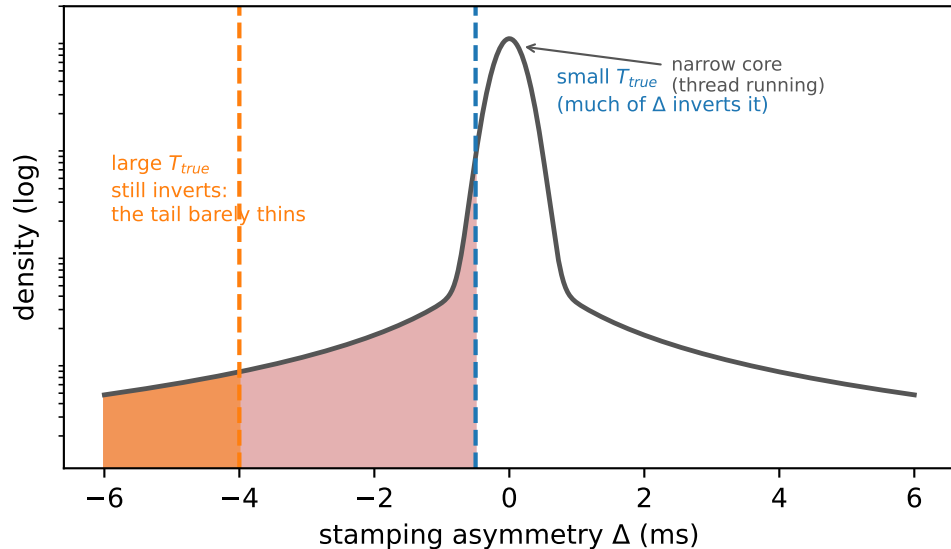
(b) a heavy tail, not a bell: P(\text{inv}) \propto T_{true}^{-0.34}
