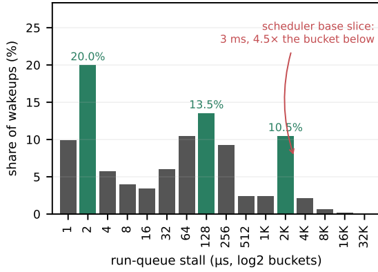
Fig. 8. The traced run-queue stall distribution is trimodal. 551,956 wakeups, bpfttrace log 2 buckets, modes shaded. The jitter core sits at a few microseconds and a second mode at 128–256 μs; the third, holding 10.5% of all wakeups, lands on the scheduler’s derived base slice of 3 ms. A power law would have to descend monotonically across this axis.
