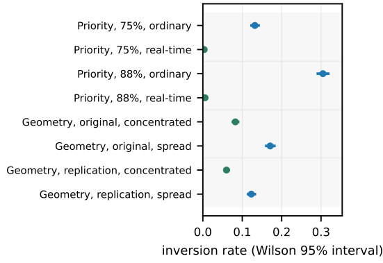
Fig. 6. Every manipulation, and no overlap. Wilson 95% intervals for the four matched pairs of Table IV: real-time priority against ordinary at two utilisations, and concentrated against spread geometry at equal \rho in two campaigns. Utilisation is held fixed within each pair, so what moves the rate is where the stamping thread sits, not how loaded the machine is.
