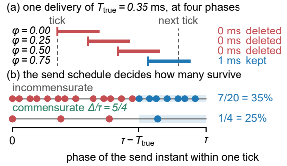
Fig. 4. Why a sample disappears, and why the survivors are not a sample . (a) One delivery of T_{\text{true}} = 0.35 ms at four phases of one tick. Three finish inside it, so both stamps round alike, the difference is exactly zero, and the guard removes them; the fourth crosses the boundary and is recorded as one whole tick — which is why the corpus prints 1.0 and 2.0 ms and nothing between. (b) A delivery survives from phase \tau - T_{\text{true}} onward — the shaded band — so uniform phases retain T_{\text{true}}/\tau (Equation 4); a commensurate producer visits only q and retains a count out of q , one of the values Equation 5 allows. T_{\text{true}} here is illustrative and off-vertex by choice: at 0.5 ms the two answers coincide.
