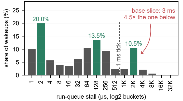
Fig. 9. The traced run-queue stall distribution is trimodal. 551,956 wakeups, bpfttrace \log_2 buckets, modes shaded. The jitter core sits at a few microseconds and a second mode at 128–256 \mu\text{s} ; the third, holding 10.5% of all wakeups, lands on the scheduler’s derived base slice of 3 ms. A power law would have to descend monotonically across this axis.
