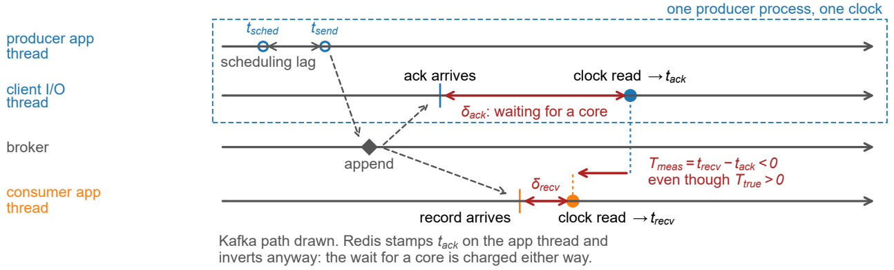
Fig. 2. A late stamp, not an early record. How a positive latency is measured as negative, on one clock. Two threads of the producer process take the two stamps — the application thread calls send, the client's I/O thread runs the delivery callback — and whichever one stamps must first be scheduled, so the difference inverts when the acknowledgment's stamping delay exceeds the true delivery plus the consumer's (Section III-A). The path drawn is Kafka's. Redis stamps on the calling thread, has no second thread, and inverts on a larger share of runs (Supplement S43.3): the wakeup is what both pay, and the hand-off only adds to it. The producer's own stamps, t_{\text{sched}} and t_{\text{send}} , do precede the acknowledgment, and the span referenced to them never inverts (Table I).
