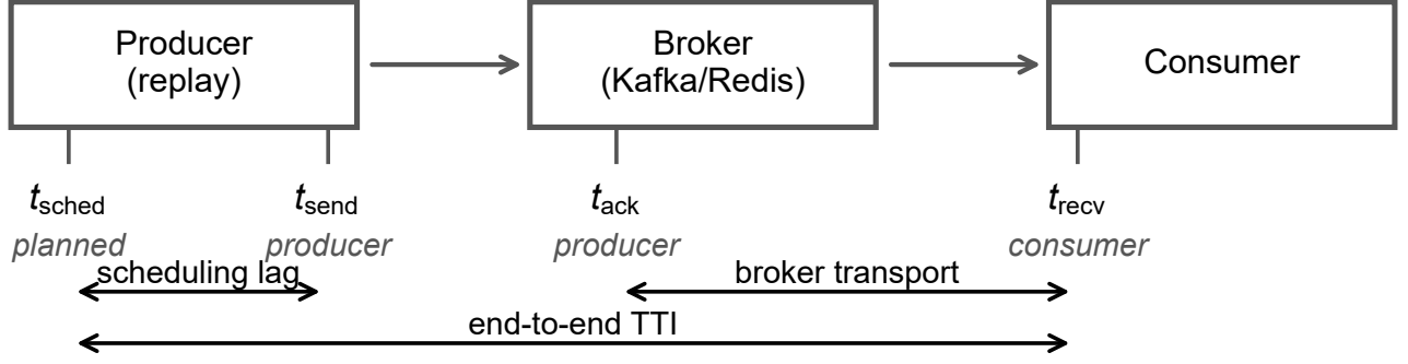
Fig. 1. The system measured, and where its clocks are read. A replay process paces recorded match events at a chosen rate into a broker — Kafka or Redis Streams — and a consumer reads them back. Four stamps are taken: t_{\text{sched}} , when an event was due; t_{\text{send}} , immediately before the send call; t_{\text{ack}} , when the producer learns the broker accepted it; and t_{\text{recv}} , when the consumer holds the record. The span this paper is about, broker transport, subtracts a stamp written in the producer process from one written in the consumer process. Both processes run on one host reading one clock unless stated otherwise (Section III-A), so nothing that follows depends on clock synchronization.
