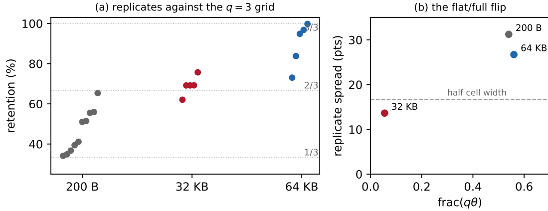
Fig. 7. The campaign’s confirmed prediction. (a) Retention replicates at 300 msg/s ( q = 3 ) by payload, against the thirds grid: 200 B straddles both branches, 32 KB pins near the 2/3 vertex, 64 KB re-opens to the upper cell. (b) Replicate spread against \text{frac}(q\theta) : the flat/full boundary at half the cell width is crossed in both directions by the one manipulated variable.
