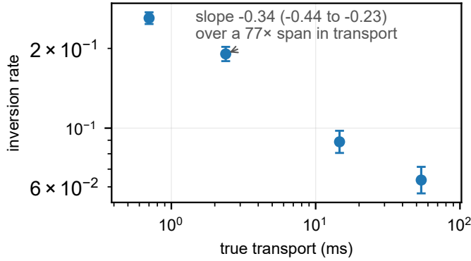
Fig. 6. A longer interval inverts less often. Inversion rate against true transport over the payload sweep, Wilson 95% intervals. The same stall distribution overlaps a short interval almost entirely and a long one hardly at all, which is Equation 3 as an experiment: lengthening what is being measured lowers the rate, where a load-driven account predicts no change.
