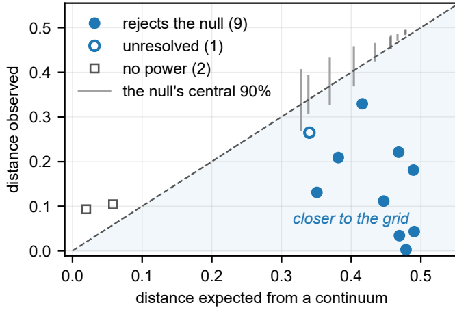
Fig. 4. Grid membership, as a set. Each configuration’s observed mean distance to the nearest grid vertex against the distance a continuum would give, which is the diagonal. The gray bar beside a configuration is its own simulated null, uncorrected ; the test is one-sided towards the grid, so a marker below its bar rejects that null. Filled circles also survive Holm correction. The open circle sits below its bar too, 0.2647 against a band opening at 0.2680, but at p = 0.044 raw and 0.131 corrected it is the one powered configuration that does not reject: correction is what the picture cannot draw. The two squares carry no bar because no test has power there: the two hypotheses coincide, and the sign carries nothing. Corrected p -values are in Supplement S23.
