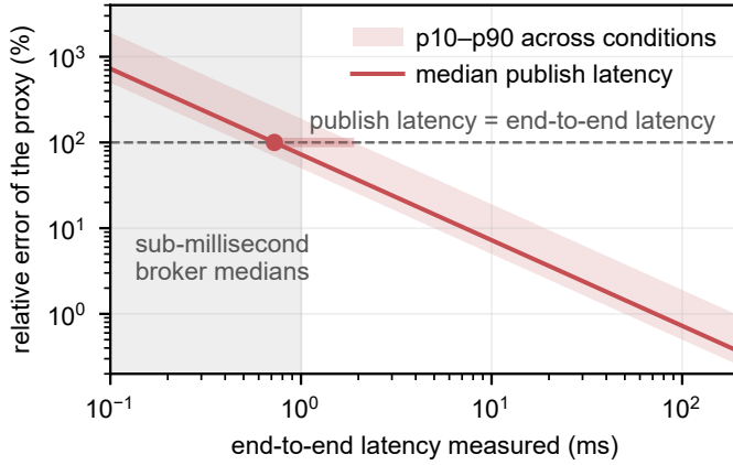
Fig. 5. Where a path sits on the exposure curve. The proxy’s error A/D against the end-to-end latency measured, the line at the median publish latency. Across conditions A runs 500–1900 \mu\text{s} between its tenth and ninetieth percentiles, the band, which puts the error at 10 ms at 5–19% and the crossover at 0.50–1.90 ms. On the dashed line, which the median crosses at 0.72 ms, the publish latency is as long as the path itself, and the shaded decade holds the sub-millisecond medians now reported for brokers. A harness that times from the publish call subtracts no publish latency and has no curve.
