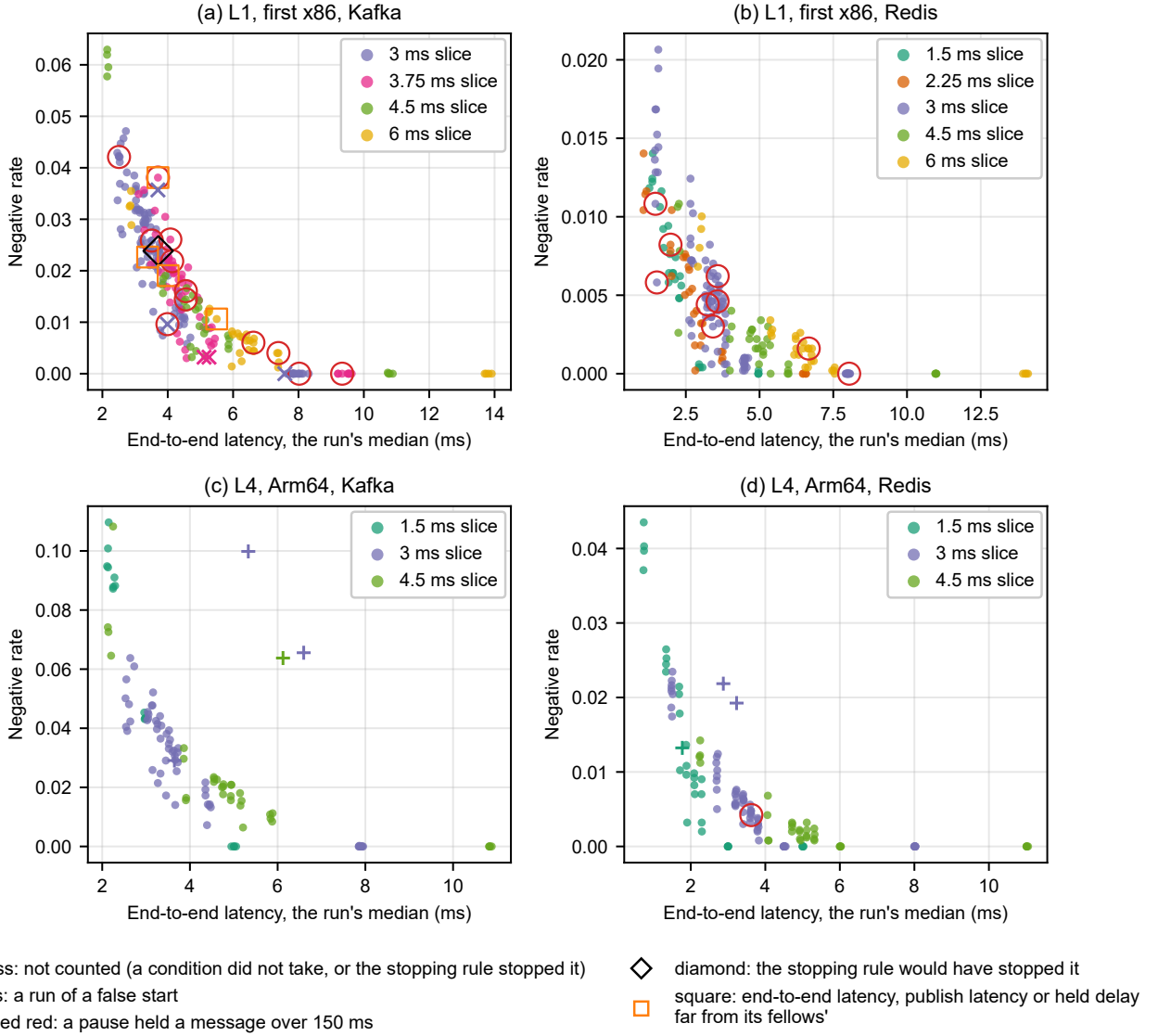
Fig. S9. Slice runs fall from the shortest end-to-end latency on, where the registered law put a plateau. Every run of L1 (first x86 pair) and L4 (Arm pair, Arm64 in the panels) at its median end-to-end latency and its negative-span rate, colored by the slice it ran at. Crosses: runs the integrity rule did not count. Plusses: runs of L4's two false starts. Rings, diamonds and squares: counted runs with a warning (S6.4). That the rate holds no plateau was read after the verdicts (S6.5).
