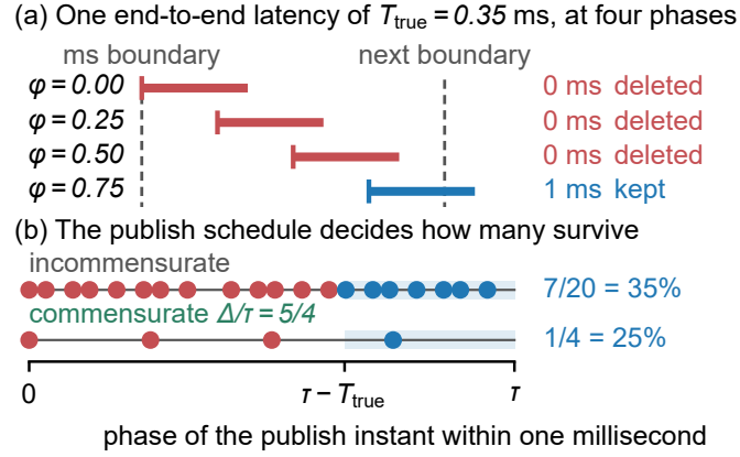
Fig. S5. Where a publish instant falls within a millisecond decides whether its sample survives. (a) One end-to-end latency of T_{\text{true}} = 0.35 ms at four phases of one millisecond. Three finish inside it, compute to zero and are removed. The fourth crosses the boundary and is recorded as one whole millisecond. (b) A sample survives from phase \tau - T_{\text{true}} onward, the shaded band, so uniform phases retain T_{\text{true}}/\tau . A commensurate producer visits only q phases and retains a count out of q . The end-to-end latency drawn is off-vertex by choice, since at 0.5 ms the two answers coincide.
