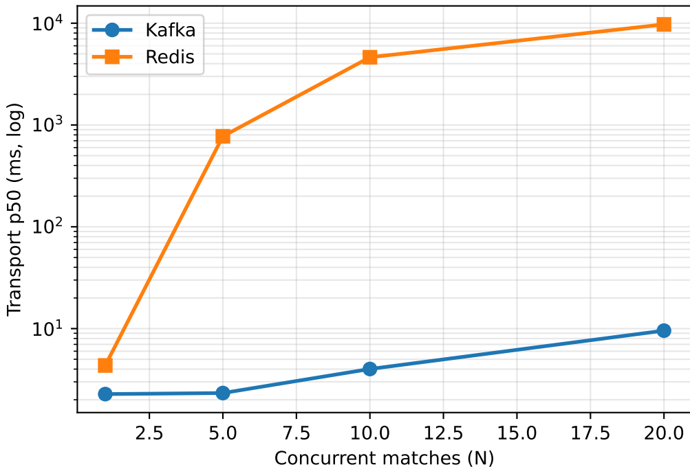
Broker transport latency vs. concurrency (single host)
