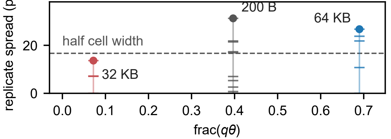
Fig. 6. The campaign's confirmed prediction. (a) Retention replicates at 300 msg/s ( q = 3 ) by payload, against the thirds grid: 200 B straddles both branches, 32 KB pins near the 2/3 vertex, 64 KB re-opens to the upper cell. Horizontal position within an arm separates replicates that would overprint and carries no variable. (b) Replicate spread against \text{frac}(q\theta) : the flat–full boundary at half the cell width is crossed in both directions by the one manipulated variable. The spread is a range, so each stick shows the replicates it is made of — 32 KB clears the boundary with three of five pinned together, 64 KB is broad.
