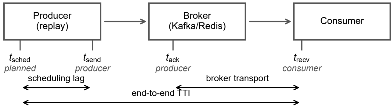
Fig. 9. The four bracketing timestamps, and the span each metric covers. Scheduling lag is measured inside one process. Broker transport subtracts a producer-side stamp from a consumer-side one, so it can come out negative when either process is delayed. A fifth stamp, t_{\text{out}} , is consumer-internal and is not drawn here; supplementary material S43.1 places it.
