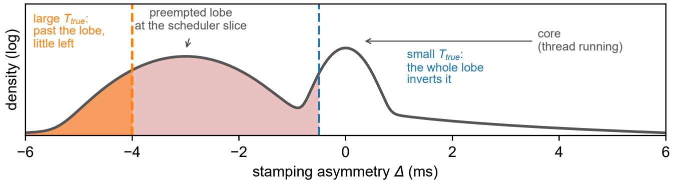
Fig. 3. The two-state model, drawn. The stamping asymmetry \Delta has a narrow core when the stamping thread is running and a lobe at -3 ms, the scheduler’s base slice, when it is not, so a small T_{\text{true}} is inverted by the whole lobe and a large one only by what lies beyond it — which is why the check bites hardest on small effects. The shape is schematic, two components placed at the measured mode’s location rather than a fit; the measured distribution is the traced stall spectrum of the main text.
