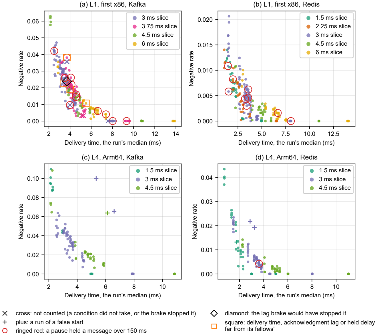
Fig. S9. Slice runs fall from the shortest delivery time on, where the registered law put a plateau. Every run of L1 (first x86 pair) and L4 (Arm pair, Arm64 in the panels) at its median delivery time and its negative-span rate, colored by the slice it ran at. Crosses: runs the integrity rule did not count. Pluses: runs of L4's two false starts. Rings, diamonds and squares: counted runs with a warning (S6.4). That the rate holds no plateau was read after the verdicts (S6.5).
