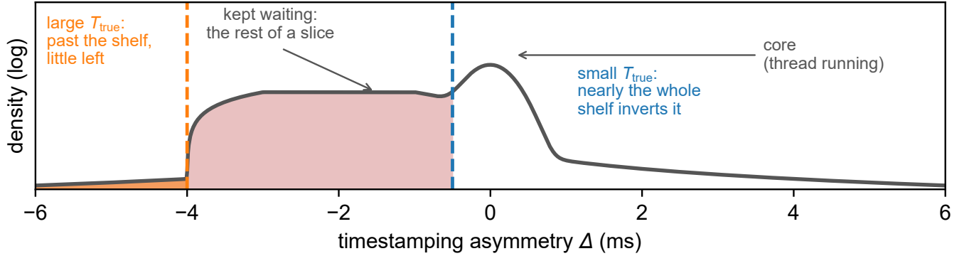
Fig. S3. In the model, a short delivery time is inverted by nearly the whole waiting state, and one longer than a slice and a tick by none of it. The two-state model, drawn. The timestamping asymmetry \Delta has a narrow core while the timestamping thread runs. While it waits, a shelf reaches from the core to -3 ms, the scheduler's base slice, and a tick beyond. The shape is schematic: two components drawn with the derived slice and tick, not fitted. The shelf, a wait for the rest of a slice, was read from the law campaign's recordings after its verdicts (S6.5). The measured distributions are the stall spectrum of Figure 3 and the per-acknowledgment waits of S6.5.
