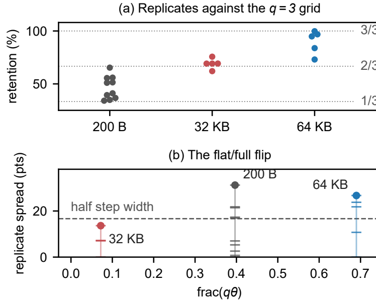
Fig. S7. One manipulated variable moves a configuration onto its lattice and off it. (a) Replicates at 300 msg/s ( q = 3 ) by payload, against the thirds lattice: 200 B straddles both branches, 32 KB pins near the 2/3 vertex, and 64 KB re-opens to the upper step. (b) Replicate spread against \text{frac}(q\theta) , each stick showing the replicates its spread is made of, with \theta each configuration's own mean retention in this campaign. The registered prediction placed 32 and 64 KB at 0.055 and 0.56 from the payload sweep's \theta . The flat–full boundary at half the step width is crossed in both directions.
