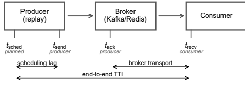
Fig. 1. The four timestamps, and the span each metric covers. Scheduling lag is measured inside one process. Broker transport subtracts a producer-side stamp from a consumer-side one, so it can come out negative when either process is delayed — which is the failure Section V takes apart.
