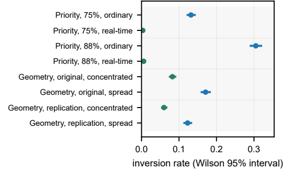
Fig. 6. Every manipulation, and no overlap. Wilson 95% intervals for the four matched pairs of Table III: real-time priority against ordinary at two utilizations, and concentrated against spread geometry at equal \rho in two campaigns. Utilization is held fixed within each pair, so what moves the rate is where the stamping thread sits, not how loaded the machine is.
