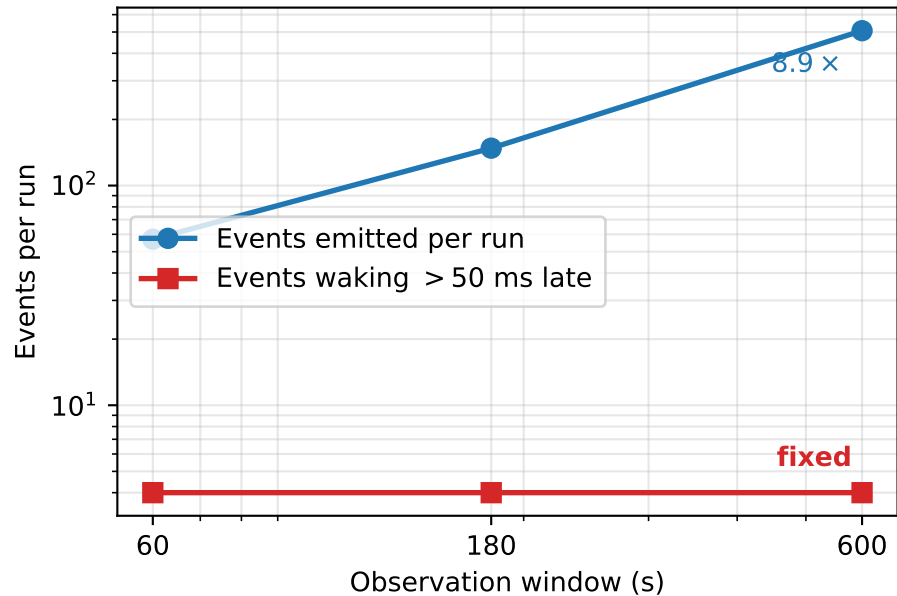
(a) One series grows, the other does not
