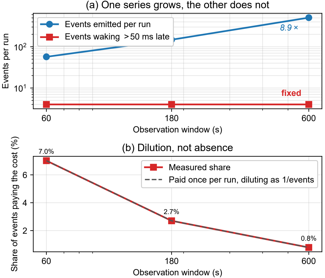
Fig. 1. The window sweep, as a picture. (a) Events emitted per run grow 8.9\times while the number waking more than 50 ms late stays at four — a per-event constant would put the two series on parallel lines. (b) The same fact as a proportion: the share of events paying the cost falls as 1/\text{events} , the dilution a once-per-run cost predicts. Redis, on the same events, has no affected events at any window.
