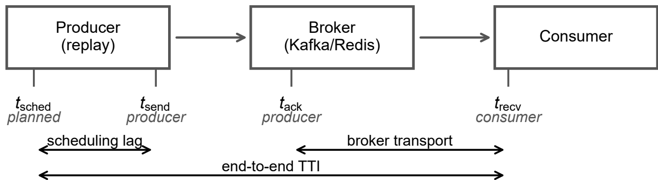
Fig. 5. The four timestamps, and the span each metric covers. Scheduling lag is measured inside one process. Broker transport subtracts a producer-side stamp from a consumer-side one, so it can come out negative when either process is delayed.
