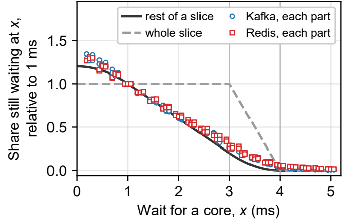
Fig. 3. Woken by the reply, a thread waits out the rest of a slice, not a whole one. For each of the registered campaign’s twelve combinations of machine pair, broker and load, the share of acknowledgments whose thread was still waiting for a core at x , relative to the share still waiting at 1 ms, over 1,516,342 acknowledgments in 304 runs. Those runs set the slice to 3 ms and the tick , the timer interval at which the kernel checks whether a slice has run out, to 1 ms. The solid curve waits out the rest of a slice and then up to a tick (Supplement S6.3); the dashed curve waits out a whole slice and a tick. The vertical lines mark the slice and a tick past it. Read after the campaign’s verdicts, on runs whose recording raised the rate it recorded 1.36- to 4.33-fold.
