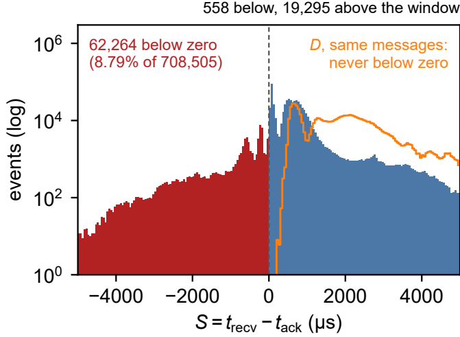
Fig. 2. S spreads over milliseconds, and part of it falls below zero. S = t_{\text{recv}} - t_{\text{ack}} for the 708,505 messages of our cloud runs on both brokers, read on one clock at nanosecond resolution and drawn in 50 \mu\text{s} bins over \pm 5 ms. The 62,264 values below zero are red; all but 558 of them lie inside the window, and 19,295 values lie above it. The orange line is D , timed from the publish call on the same messages, which is never below zero.
