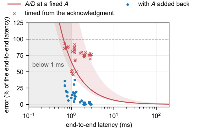
Fig. 5. Adding the publish latency back repairs the latency. The error of S as a latency on each of our 70 groups of runs, one per condition and sign-check verdict (crosses), and once the publish latency is added back (dots), against the group's end-to-end latency. The curve is A/D for one path at the median publish latency, and its band covers the tenth to ninetyth percentiles of A across groups, 500\text{--}1900\ \mu\text{s} . The crosses sit above it because the conditions with a longer end-to-end latency also have a longer publish latency. On the dashed line A equals D . The shaded decade holds the sub-millisecond medians now reported for brokers.
