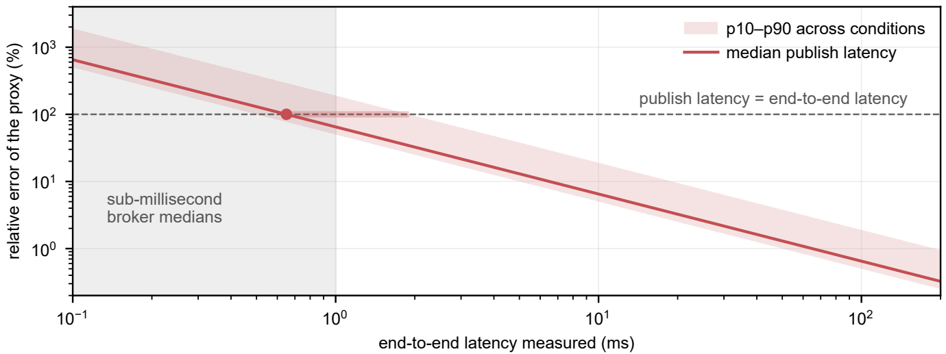
Fig. S9. Where a path sits on the exposure curve. Table S9 as a curve: the relative error of the acknowledgment-timed proxy, A/T_{\text{true}} , against the end-to-end latency measured. The line is this corpus’s median publish latency and the band its tenth to ninetieth percentile across conditions, so a reader can bracket their own path rather than take the middle. The bar on the dashed line is the crossover, where the publish latency equals the end-to-end latency it is a correction to: 0.65 ms at the median publish latency and 1.90 ms at the ninetieth percentile, marked as an interval because it is one. To its left the correction is larger than the quantity corrected. The shaded column is where published broker medians sit (Section S33.4), which is the reason the curve matters.
