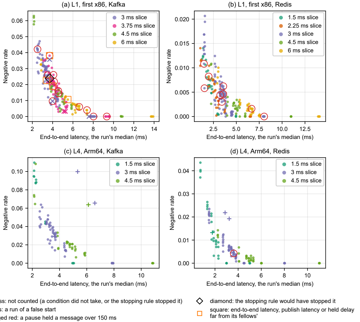
Fig. S17. Every slice run, aberrant runs marked. Each run of L1 (first x86 pair) and L4 (Arm pair, Arm64 in the panels) at its median end-to-end latency and its negative-span rate, colored by the slice it ran at. Crosses: runs the integrity rule did not count. Plusses: runs of L4's two false starts. Rings: counted runs with a warning, each reason its own shape (Table S32).
