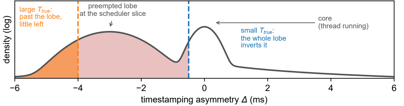
Fig. 4. The two-state model, drawn. The timestamping asymmetry \Delta has a narrow core when the timestamping thread is running and a lobe at -3 ms, the scheduler's base slice, when it is not, so a small T_{\text{true}} is inverted by the whole lobe and a large one only by what lies beyond it — which is why the check bites hardest on small effects. The shape is schematic, two components placed at the measured mode's location rather than a fit; the measured distribution is the traced stall spectrum of the main text.
