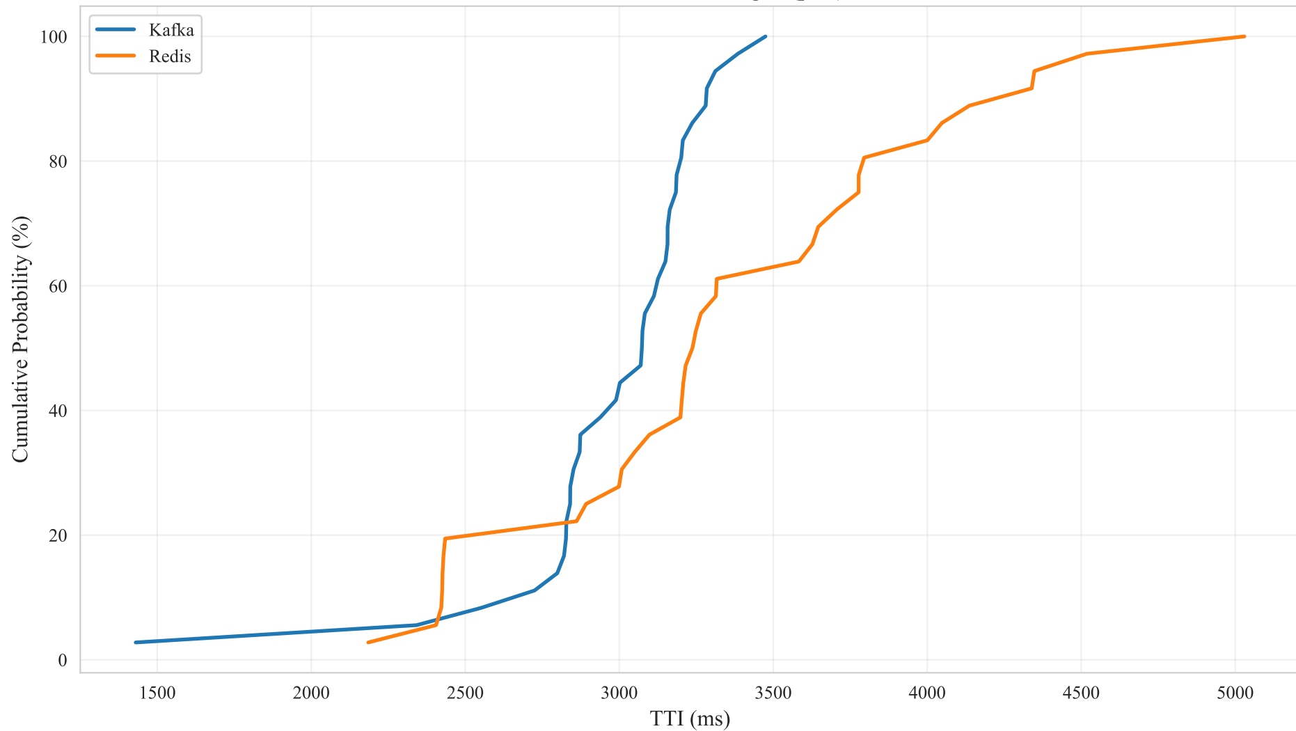
CDF of Time-to-Insight (p50)
