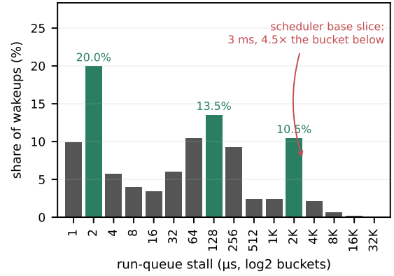
Fig. 8. The traced run-queue stall distribution is trimodal. 551,956 wakeups, bpfttrace \log_2 buckets, modes shaded. The jitter core sits at a few microseconds and a second mode at 128–256 \mu\text{s} ; the third, holding 10.5% of all wakeups, lands on the scheduler’s derived base slice of 3 ms. A power law would have to descend monotonically across this axis.
