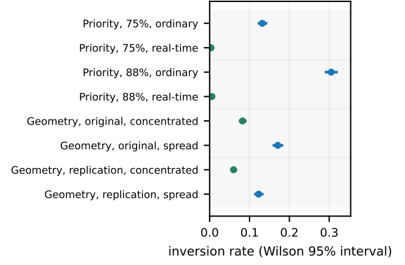
Fig. 6. Every manipulation, and no overlap. Wilson 95% intervals for the four matched pairs of Table IV: real-time priority against ordinary at two utilisations, and concentrated against spread geometry at equal \rho in two campaigns. Utilisation is held fixed within each pair, so what moves the rate is where the stamping thread sits, not how loaded the machine is.
