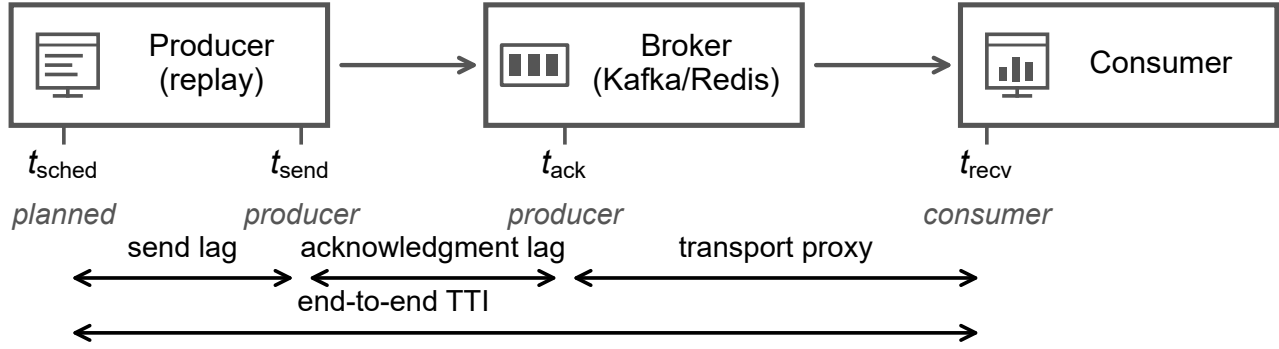
Fig. S16. System measured, and where its clocks are read. A replay process paces recorded match events at a chosen rate into a broker — Kafka or Redis Streams — and a consumer reads them back. The four timestamps and the four spans they bracket are those of main-text Section II-A; the upper three are the terms of Equation 2 and sum to the fourth. The transport proxy subtracts a producer-process timestamp from a consumer-process one. Both processes run on one host reading one clock unless stated otherwise, so nothing drawn here depends on clock synchronization.
