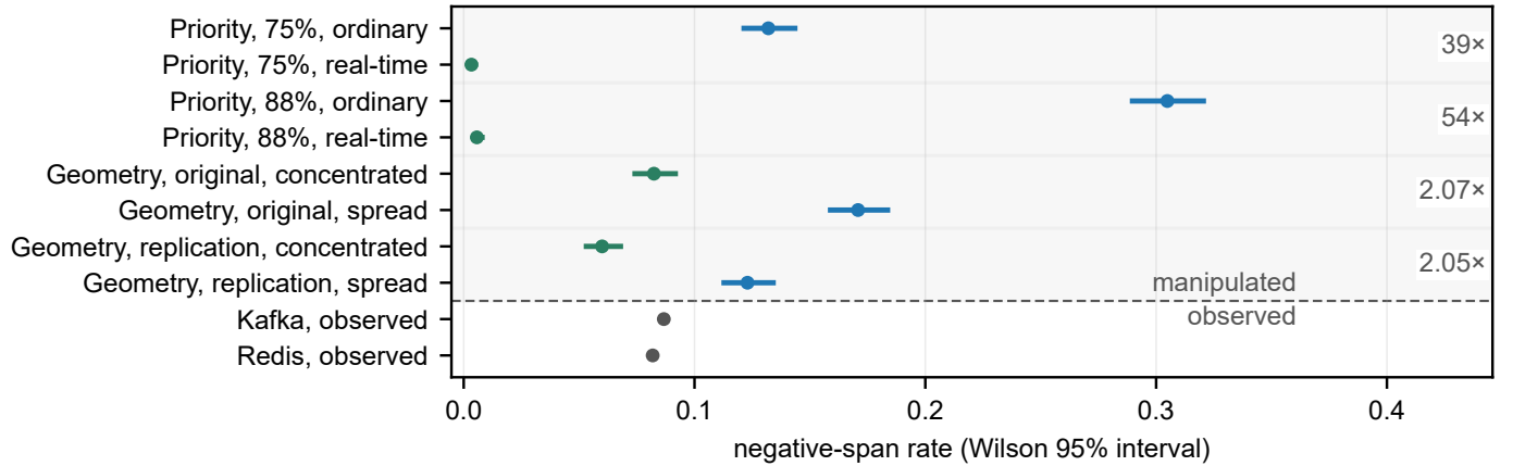
Fig. S8. Every manipulation separates; the broker does not. Wilson 95% intervals. Above the rule, the four matched pairs of Table II, utilization held fixed within each: what moves the rate is where the timestamping thread sits, not how loaded the machine is. Below it, observed rather than manipulated, the two brokers of Table I; their intervals are narrower than the plotted point.
