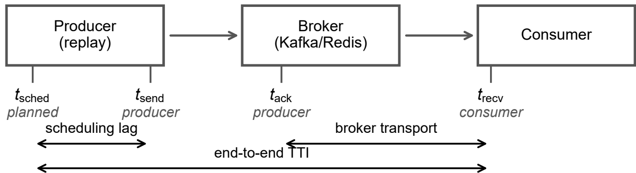
Fig. 6. The four timestamps, and the span each metric covers. Scheduling lag is measured inside one process. Broker transport subtracts a producer-side stamp from a consumer-side one, so it can come out negative when either process is delayed.
