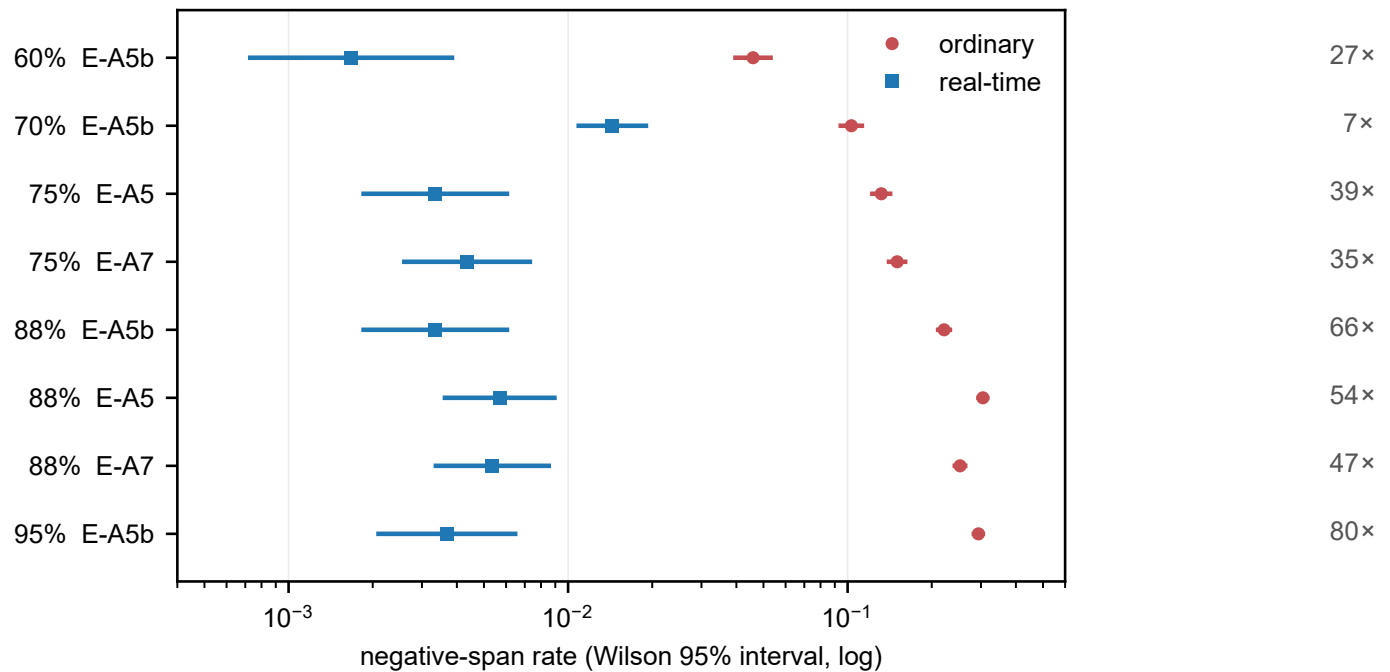
Fig. 7. The same 8 pairs, as a ladder. Ordinary and real-time negative-span rates with Wilson 95% intervals, one row per pair, ordered by achieved utilization; the factor is printed at the right. Reading down, the real-time arm barely moves while the ordinary arm climbs with load, which is what makes the factor grow. The growth is a trend and not a law — 60% gives 27\times and 70% gives 7\times — and the range is reported as a range for that reason.
