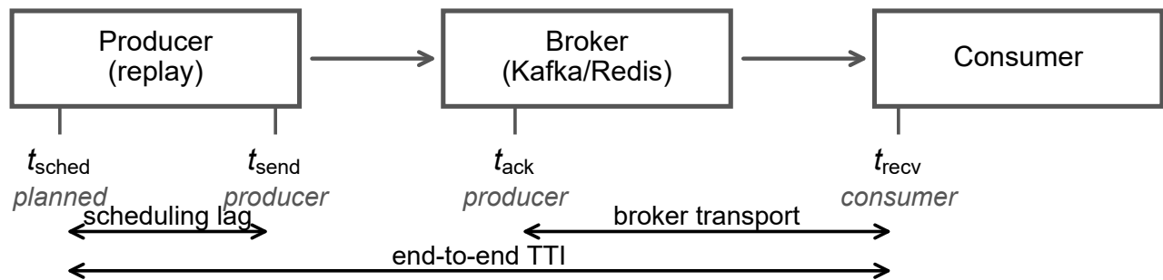
Fig. 6. The four timestamps, and the span each metric covers. Scheduling lag is measured inside one process. Broker transport subtracts a producer-side stamp from a consumer-side one, so it can come out negative when either process is delayed.
