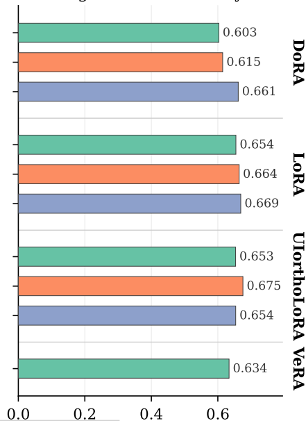
Avg General Accuracy
