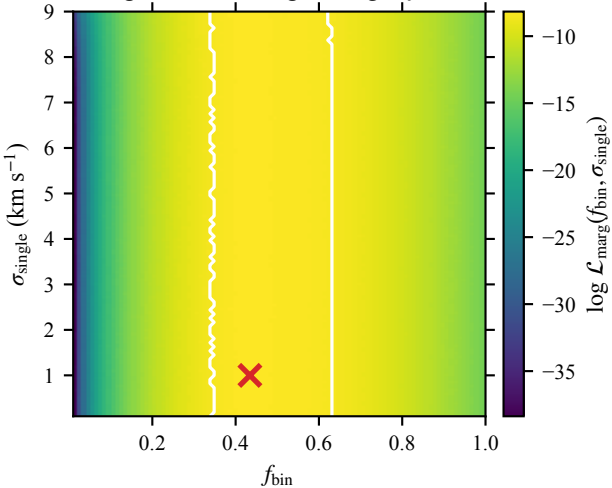
Langer model: marginal \log \mathcal{L}(f_{\text{bin}}, \sigma)
