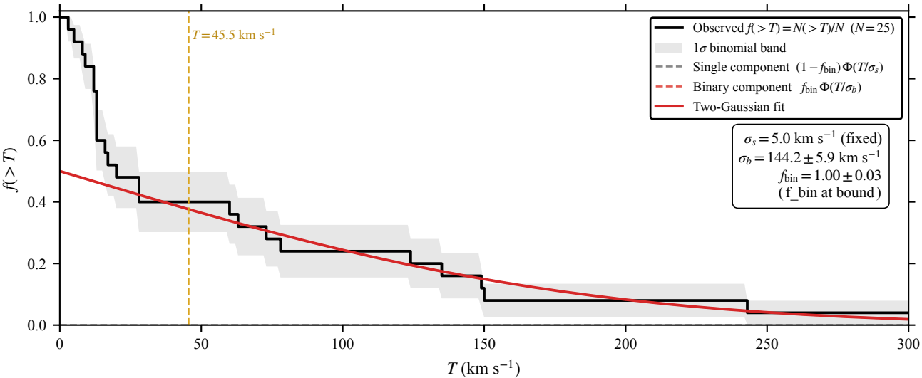
Cumulative \Delta RV distribution and two-Gaussian fit
