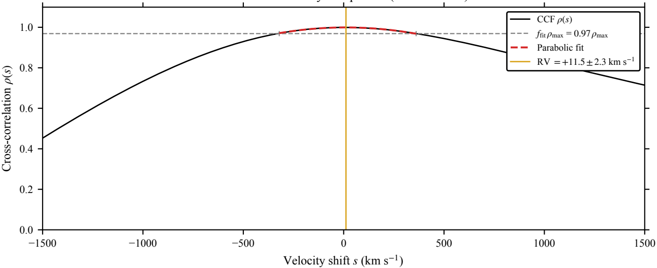
Worked CCF: Brey 93 epoch 2 (C IV 5808 Å)
