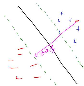
Figure 7.12: one bad point with slack
