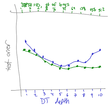
Figure 13.2: graph depicting overfitting using regularization versus bagging
