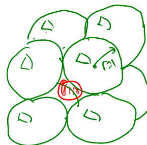
Figure 3.17: 3d spheres in spheres
