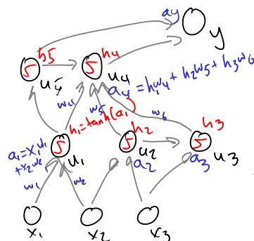
Figure 10.5: DAG network
