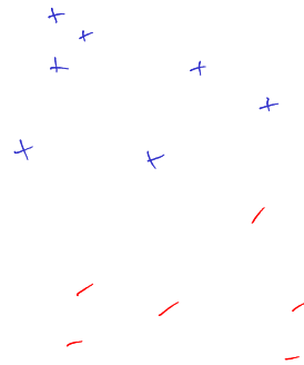
Figure 4.10: separable data
