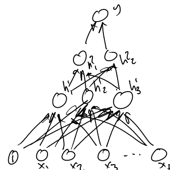
Figure 10.4: multi-layer network
