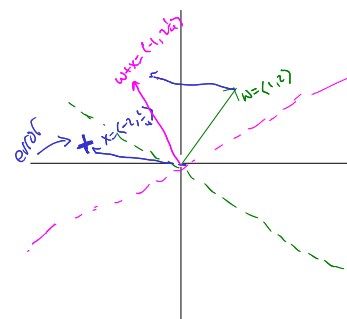
Figure 4.8: perc:bias: perceptron picture with bias
