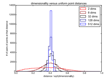
Figure 3.18: histogram of distances in D=2,8,32,128,512
