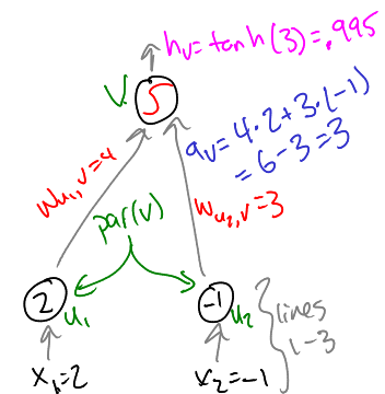
Figure 10.6: picture of forward prop
