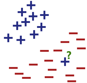
Figure 3.4: A figure showing an easy NN classification problem where the test point is a ? and should be positive, but its NN is actually a negative point that's noisy.
