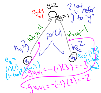
Figure 10.7: picture of back prop
