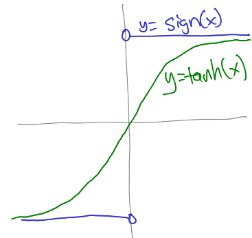
Figure 10.2: picture of sign versus tanh
