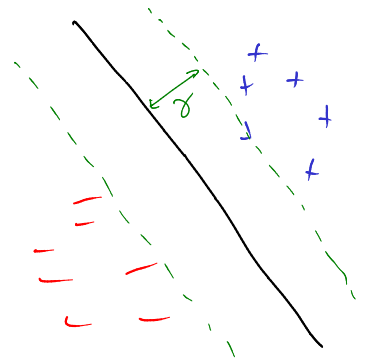
Figure 7.11: hyperplane with margins on sides
