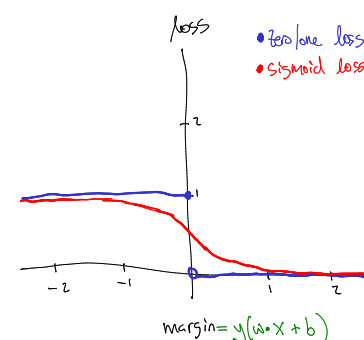
Figure 7.2: plot of zero/one versus margin and an S version of it
