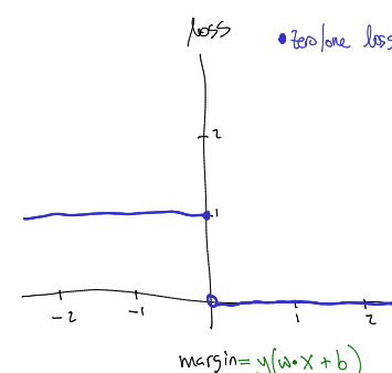
Figure 7.1: plot of zero/one versus margin
