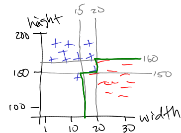
Figure 3.12: decision boundary for dt in previous figure
