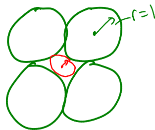
Figure 3.16: 2d spheres in spheres
