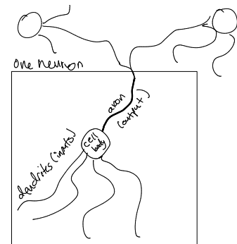
Figure 4.1: a picture of a neuron
