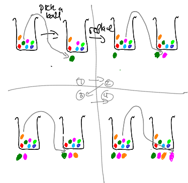
Figure 13.1: picture of sampling with replacement
