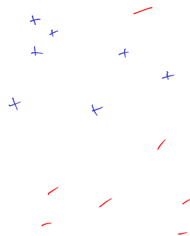
Figure 4.11: inseparable data
