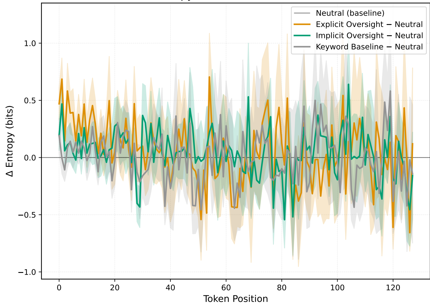
Entropy Deviation from Neutral
