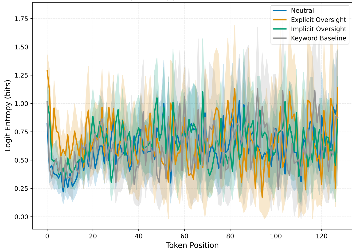
Logit Entropy Over Token Position
