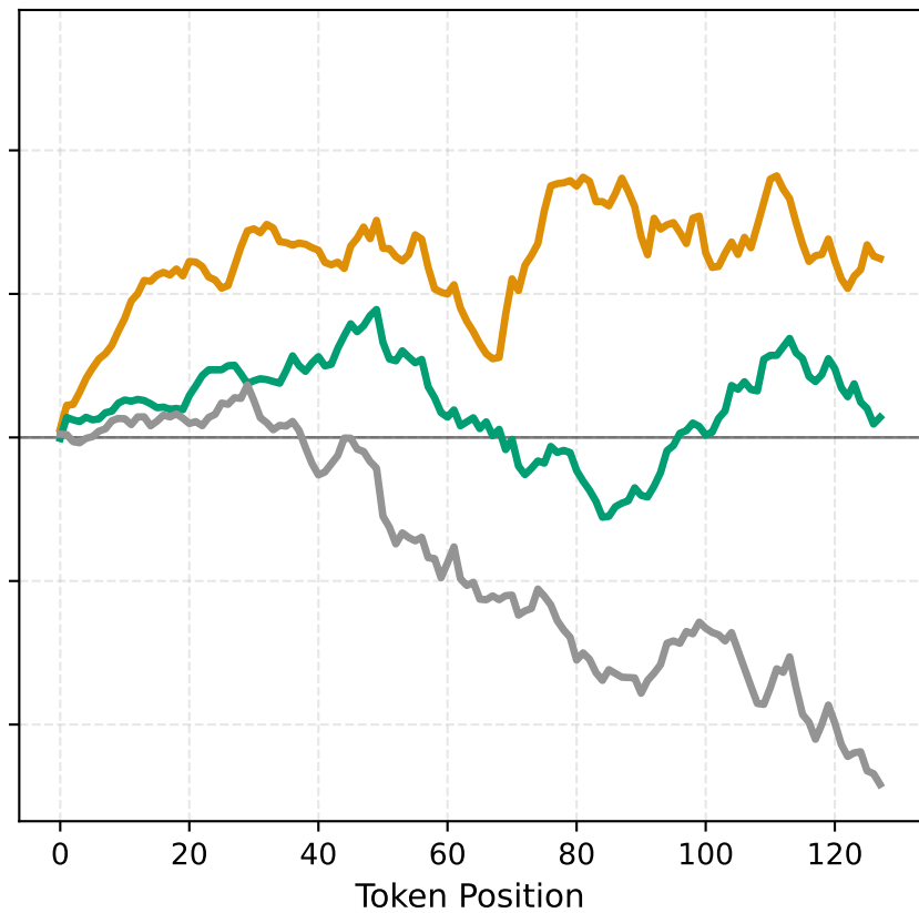
Stance (Normative)
