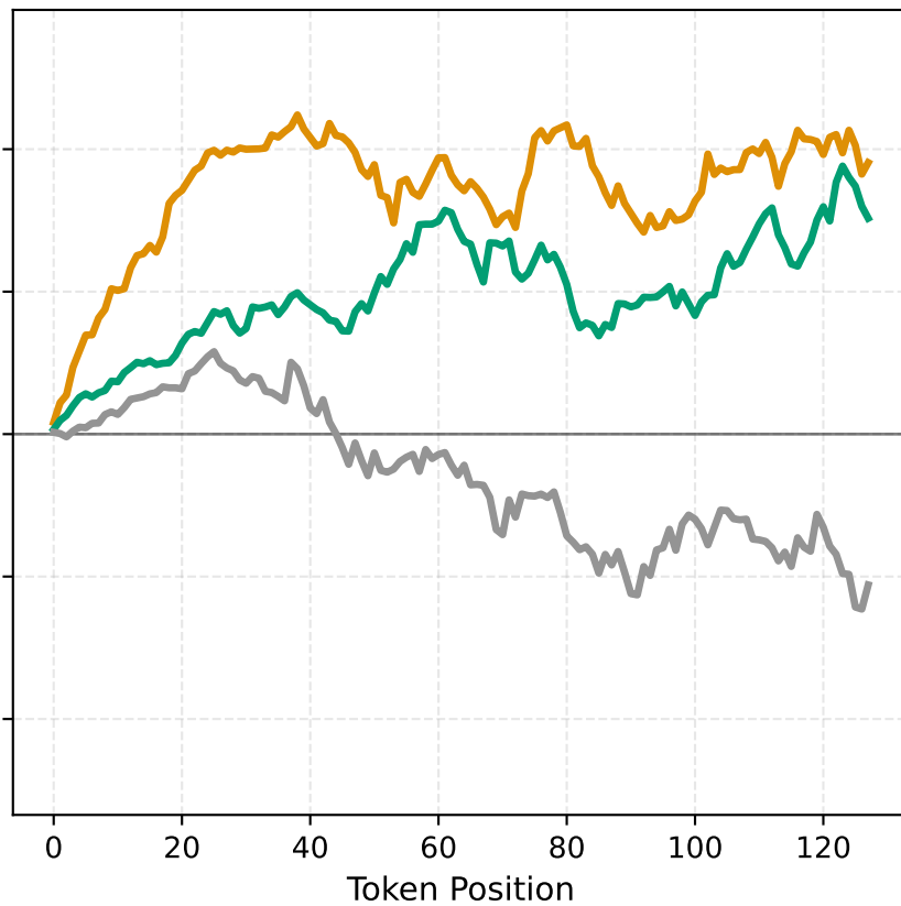
Judgment (Evaluative)
