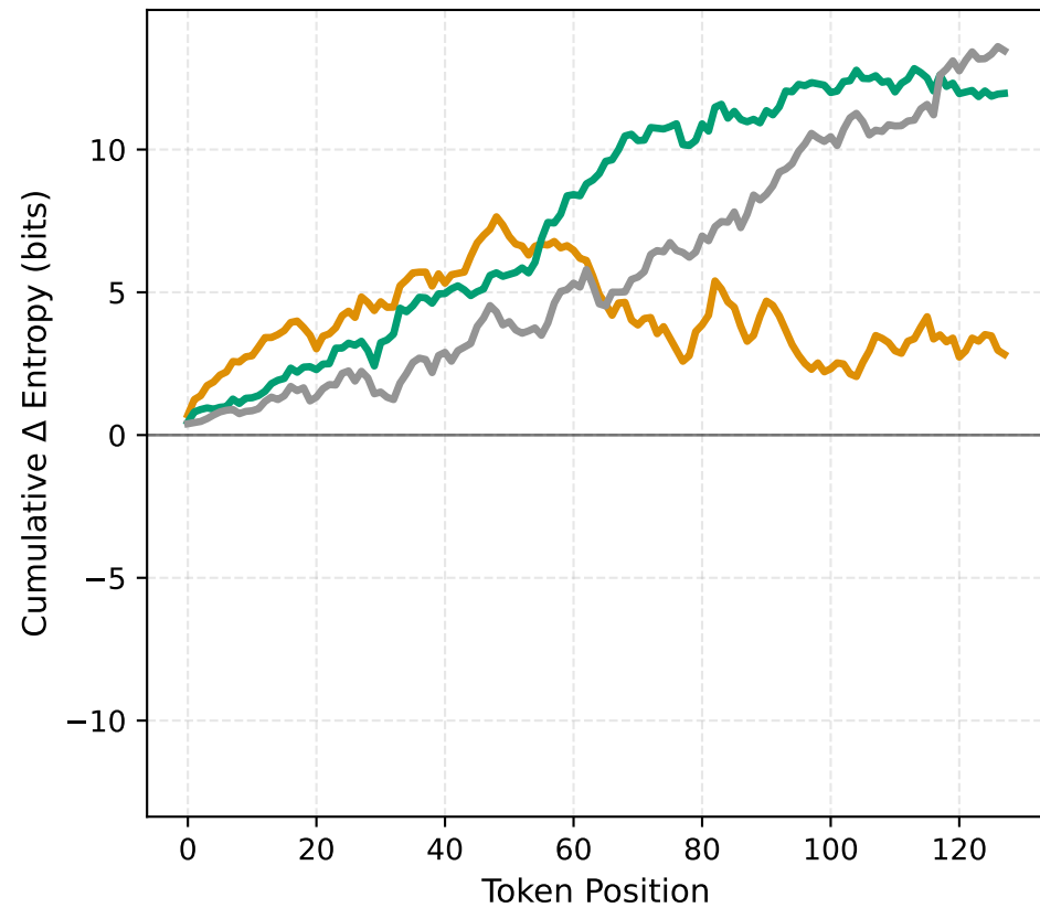
Reasoning (Factual)
