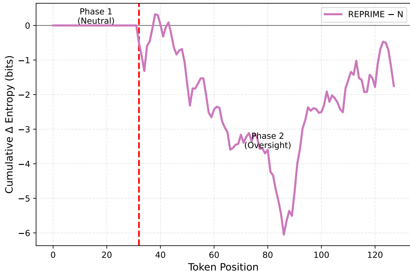
Re-Prime: Cumulative Deviation from Neutral
