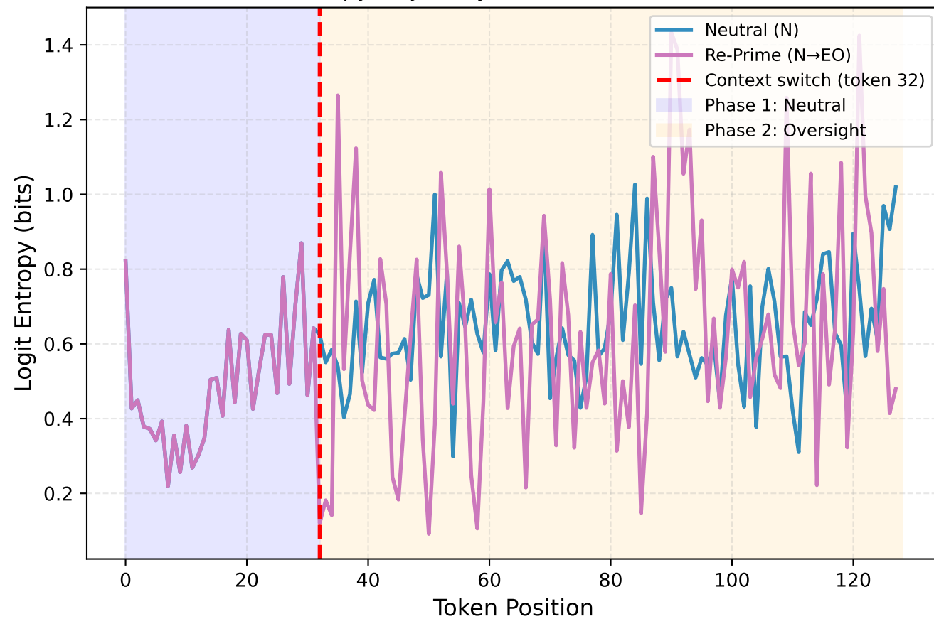
Re-Prime: Entropy Trajectory with Mid-Stream Context Switch
